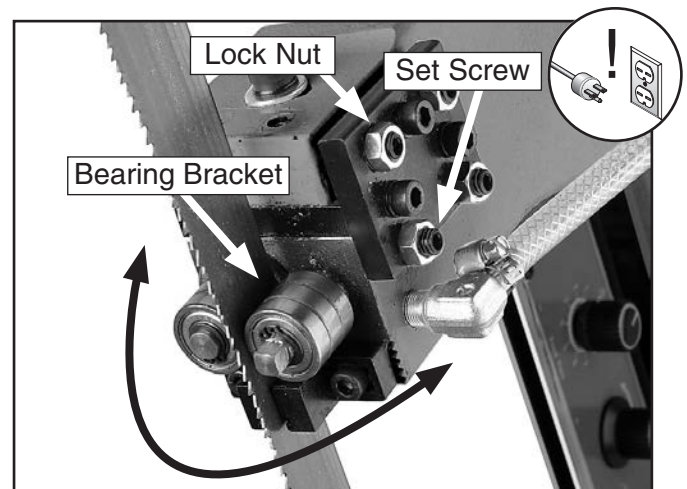
Figure 46. Bearing block pivot.
